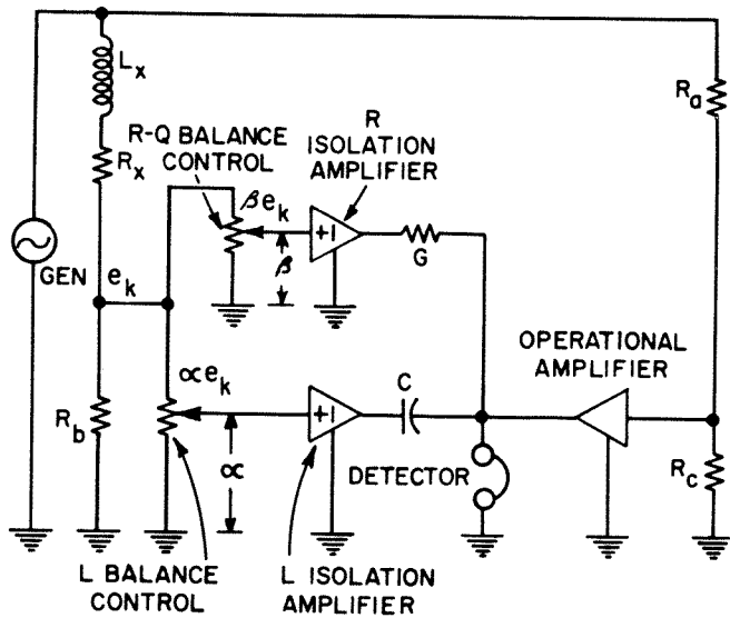
Figure 3-2. Simplified circuit for the R balance control.
