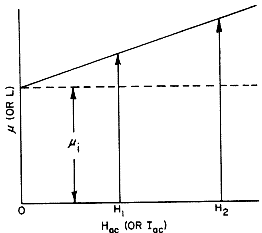
Figure 4-1. Determination of initial permeability.
