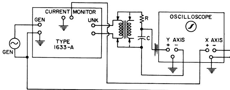
Figure 5-7. Method of displaying an ac hysteresis loop on an oscilloscope.
