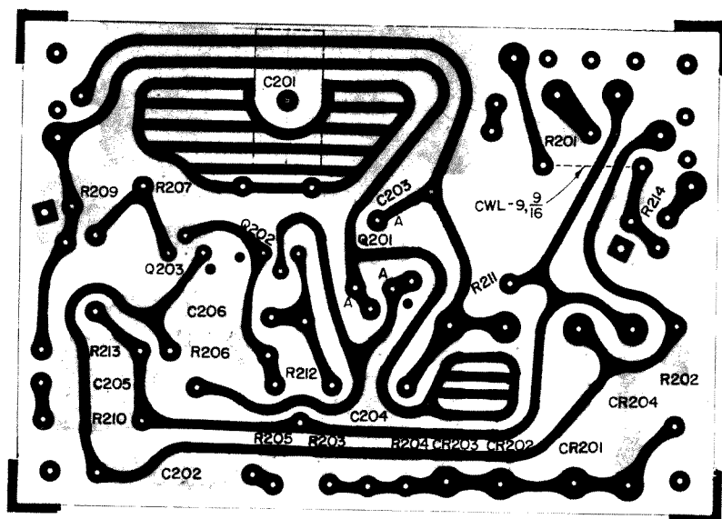
Figure 6-4. Etched board layout of isolating amplifier.
