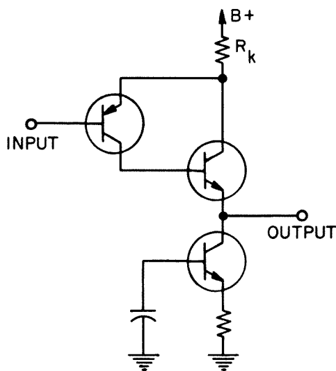
Figure 3-5. Simplified diagram of the operational amplifier.
