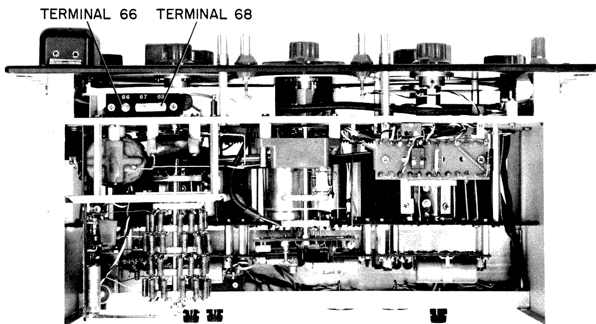
Figure 6.2. Top interior view.
