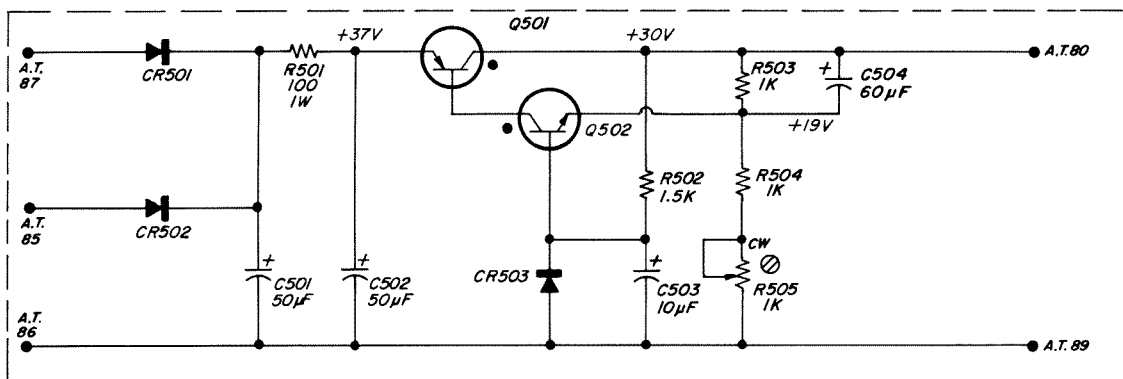
Figure 6-7. Schematic diagram of power supply.
