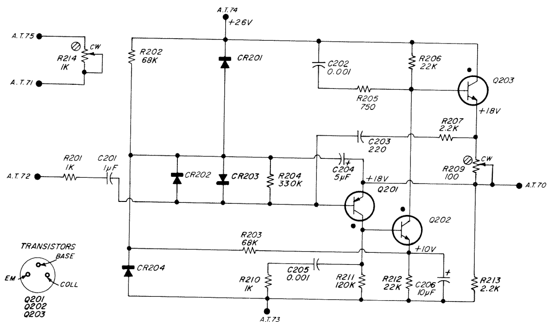
Figure 6-3. Schematic diagram of isolating amplifier.
