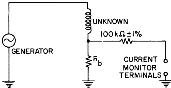
Figure 2-1. Connections to the CURRENT MONITOR panel terminals.
