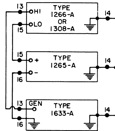
Figure 1-3. Block diagram of Type 1630 Inductance Measuring Assemblies showing interconnections.
