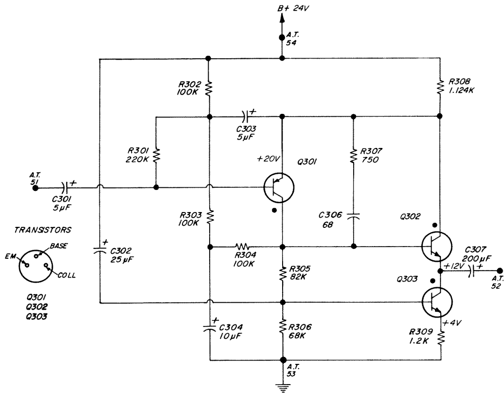
Figure 6-5. Schematic diagram of operational amplifier.
