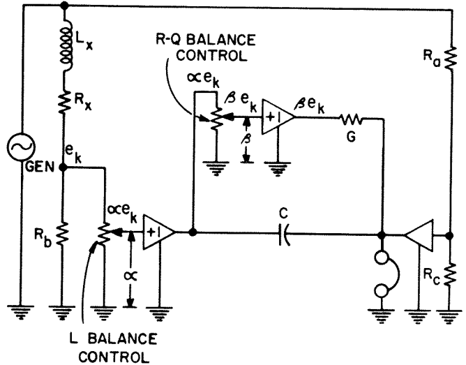
Figure 3-3. Simplified circuit for the Q balance control.
