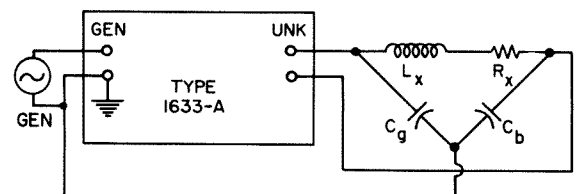
Figure 5-2. Diagram of connections for three-terminal measurements.
