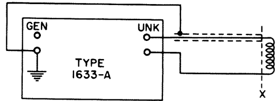
Figure 5-4. Use of a shielded cable to connect the unknown to the bridge.
