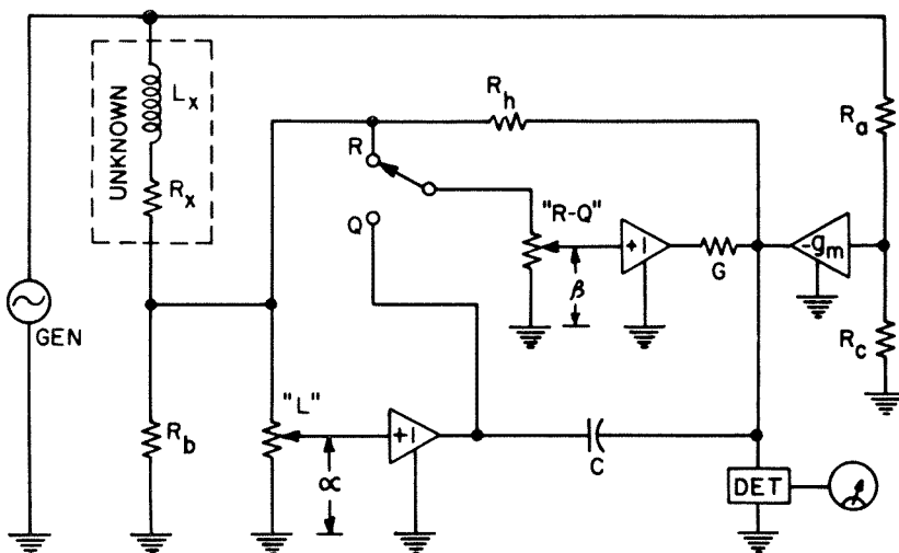
Figure 3-1. Elementary schematic diagram for Type 1633-A Incremental Inductance Bridge.
