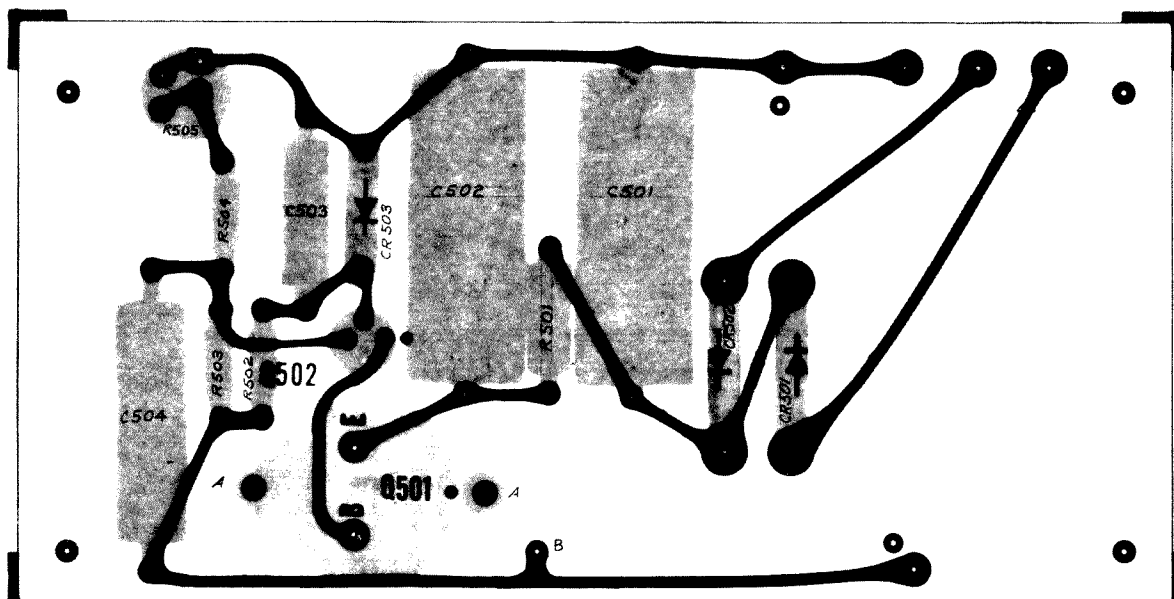
Figure 6-8. Etched board layout of power supply.
