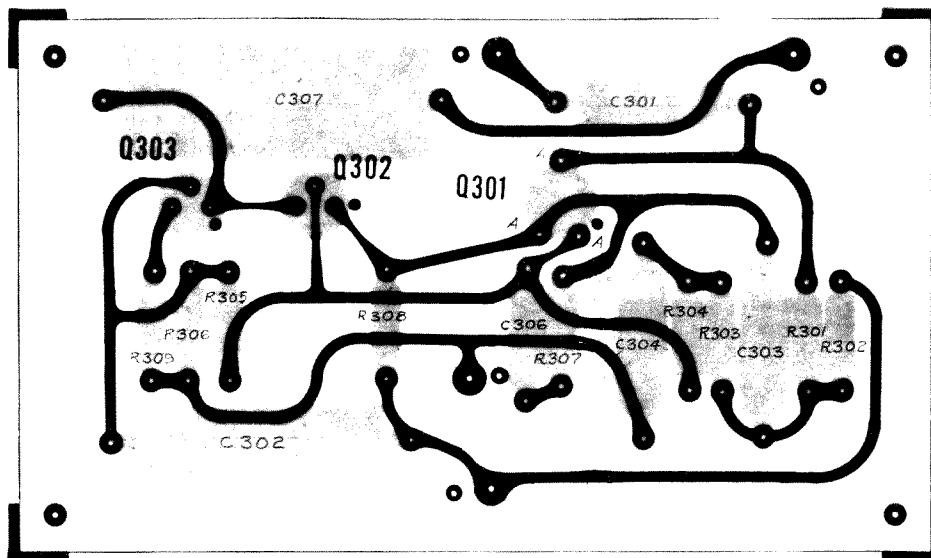
Figure 6-6. Etched board layout of operational amplifier.
