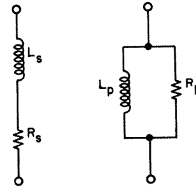
Figure 1-2. Equivalent circuits for a complex impedance.
