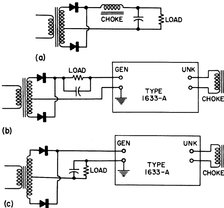
Figure 5-3. a, b, and c. A typical power supply circuit (a) and two possible methods for measurement of the filter choke (b and c).
