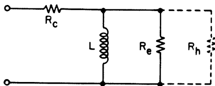
Figure 4-2. Equivalent circuit of an iron-cored coil at low frequencies.
