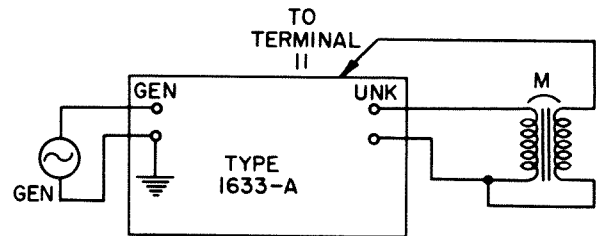
Figure 5-5. Connections for measurement of mutual inductance.
