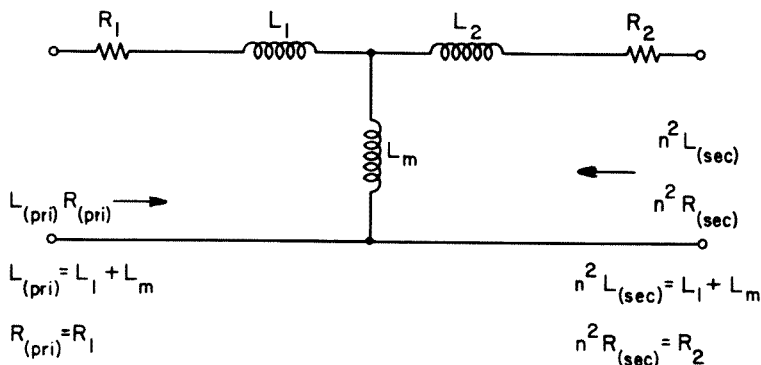
Figure 4-4. The equivalent circuit of a transformer at low frequencies.
