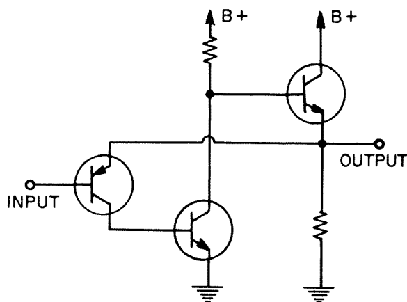
Figure 3-4. Simplified diagram of the isolation amplifier.
