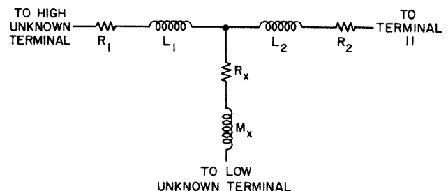
Figure 5-6. Equivalent circuit of mutual inductance.
