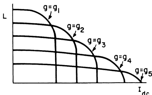
Figure 4-5. Use of optimum-size air gap in an inductor carrying a given value of direct current to produce maximum value of inductance of the coil.
