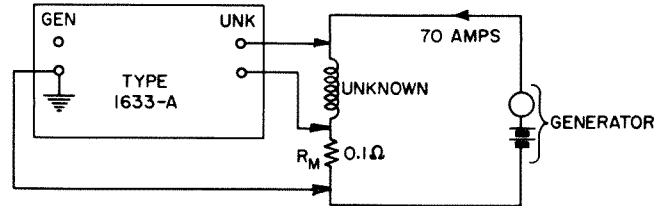
Figure 5-1. Circuit showing addition of 0.1-ohm resistor for measurements involving higher current values.
