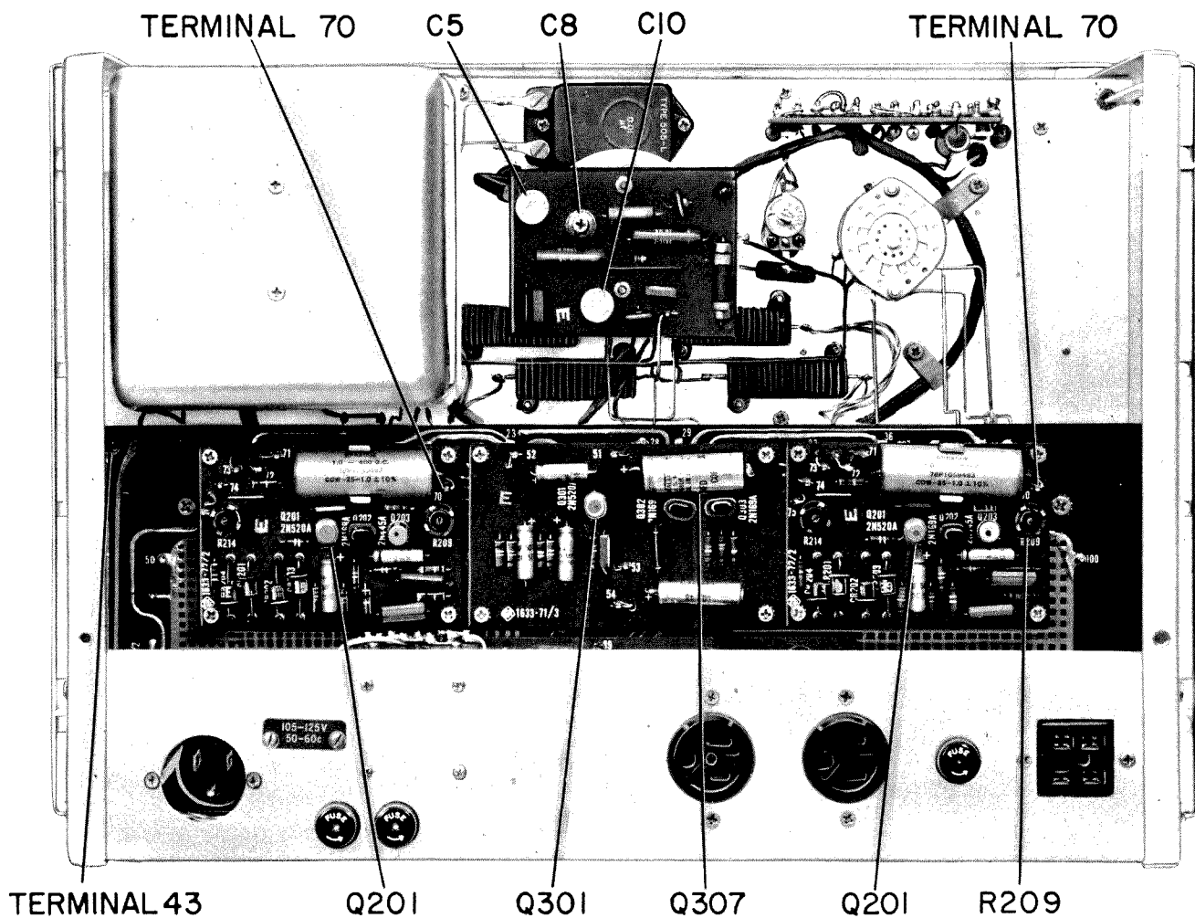
Figure 6-1. Rear interior view.
