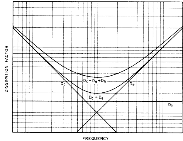
Figure 4-3. Curves showing relationships between dissipation factor and frequency. The three labeled straight lines are separate dissipation factor curves.
