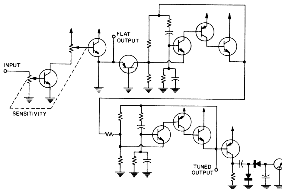
Figure 3-6. Simplified diagram of the internal detector.
